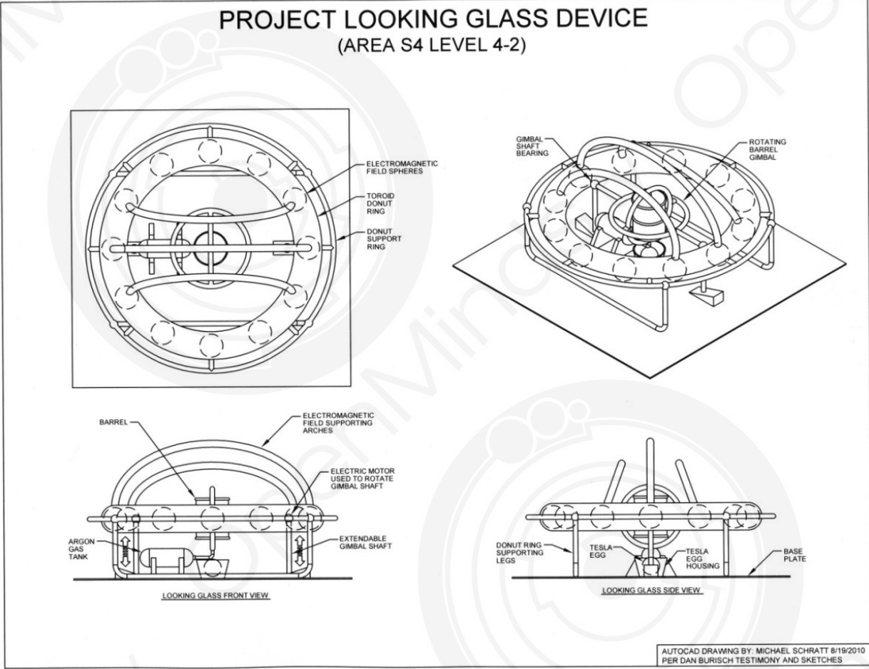
Three-view drawing of the Looking Glass device.*
